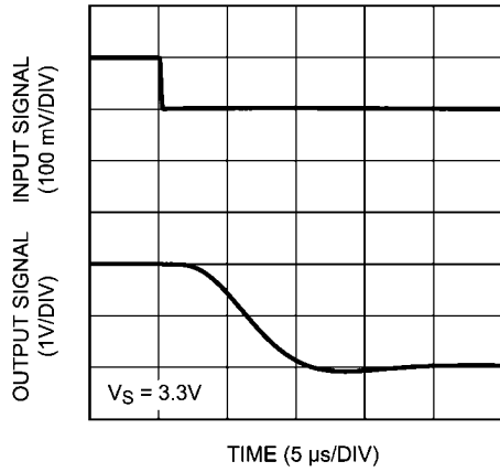
Settling Time (Falling Edge) at V_S = 3.3V
